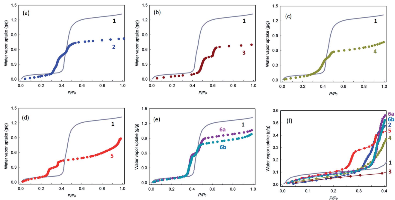
Fig. 4 Water adsorption branch isotherms measured at 298 K for (a) MIL-101-NH 2 (2), (b) MIL-101-pUR2 (3), (c) MIL-101-pMal (4), (d) MIL-101-p3SO 3 H (5), and (e) MIL-101-pCOOH (6a and 6b) compared with that of MIL-101 (1). (f) Water adsorption isotherms for 1–6 displayed together for comparison of the low pressure region. Full adsorption and desorption isotherms are presented in the ESI.†
