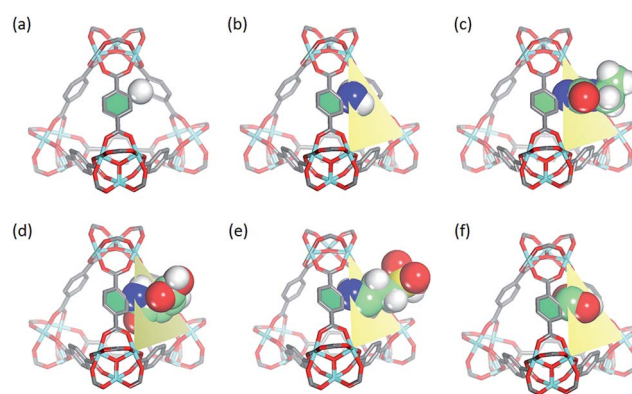
Fig. 5 Comparison of the functional groups and their possible locations on the face of a geometry-optimized ST unit drawn with space-filling models: (a) –H, (b) –NH 2 , (c) –UR2, (d) –Mal, (e) –3SO 3 H, and (f) –COOH. The STs for MIL-101 and MIL-101-NH 2 are not displayed separately because non-H functional groups give many possible locations and raise complexity. The trigonal faces are defined by three Cr ions at the ST vertices. All H atoms except for those in the functionalities are omitted, and the oxygen atoms bonded to the Cr centres are also not shown for clarity. The C atoms in the functional groups are highlighted with light green colour.
