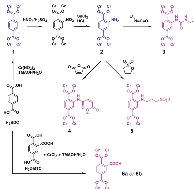
Scheme 1 The preparation of MIL-101 and its derivatives in this work are schematically drawn. MIL-101 derivatives containing two kinds of functional groups in the framework are highlighted with pink colour. TMAOH stands for tetramethylammonium hydroxide.
