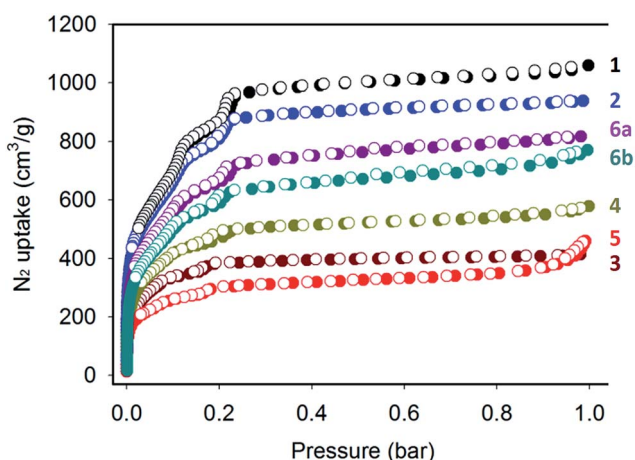
Fig. 3 Nitrogen adsorption (filled circles) and desorption (open circles) isotherms measured at 77 K for MIL-101 (1), (b) MIL-101-NH 2 (2), MIL-101- \rho UR2 (3), MIL-101- \rho Mal (4), MIL-101- \rho 3SO 3 H (5), and MIL-101- \rho COOH (6a, 6b).
