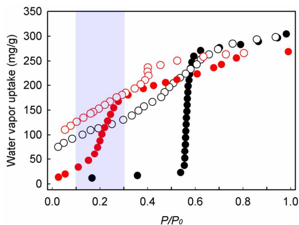
Fig. 4 Water vapour adsorption isotherms of UiO-67 (black) and UiO-67-(NH 2 ) 2 (red) measured at 298 K. The optimal P/P_0 range ( P/P_0 = 0.1 –0.3) is highlighted with a blue block; P_0 : 3.169 kPa. The adsorption and desorption branches are represented by filled and open circles, respectively.
