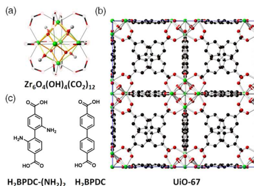
Fig. 1. (a) Inorganic secondary building unit of UiO-67. (b) The crystal structure of UiO-67. (c) Linear linker (H 2 BPDC) for the preparation of UiO-67 and its amine-functionalized form (H 2 BPDC-(NH 2 ) 2 ) for UiO-67-(NH 2 ) 2 . In (a), Zr ions and hydroxyl H atoms are displayed as green and grey balls, respectively. C and O atoms are depicted as black and red balls, respectively.
