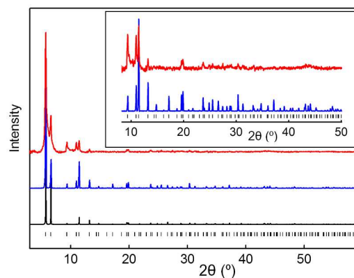
Fig. 2 The PXRD patterns of UiO-67 (blue) and UiO-67-( \text{NH}_2 ) 2 (red) are compared to a simulated pattern (black) generated from the crystal structure of UiO-67. The inset shows a magnified region of the patterns. Fig. S3 shows these patterns in a full 2 \theta range.
